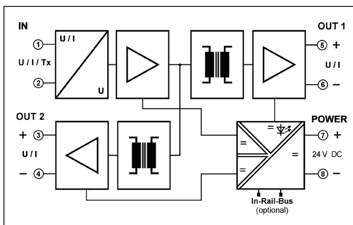
Block diagram
